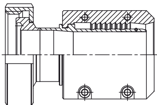
Hose connection acc. to DIN 11864-1 (Male ferrule)
