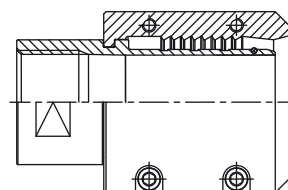
Hose connection with internal thread (Gas pipe thread cyl. acc. to ISO 228-1)
