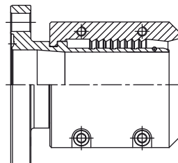
Hose connection acc. to DIN 11864-3 (Male ferrule)
