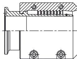
Hose connection acc. to DIN 11851 (Female ferrule threaded)
