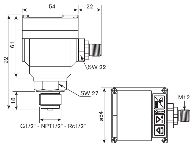
Transmitter / Switch M12 plug
