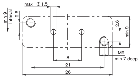
2/2 way connection
