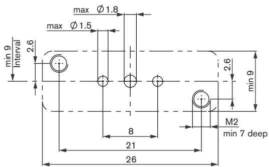
3/2 way connection
