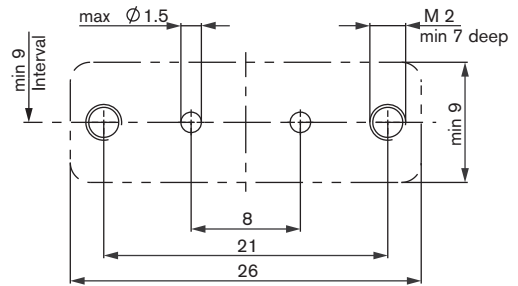
3/2 way connection
