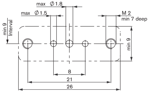
3/2 way connection
